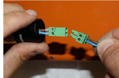
Blue -> blue Brown -> brown
